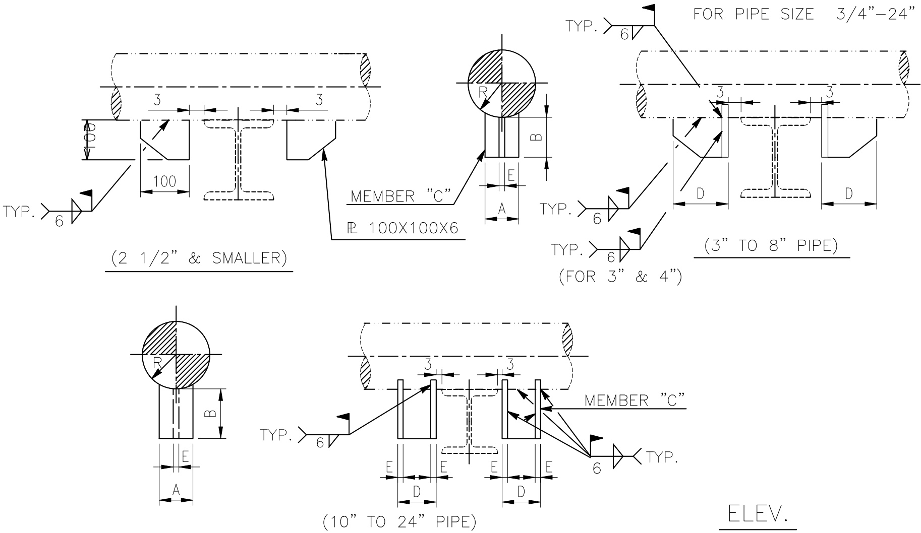
DIMENSION (mm)
