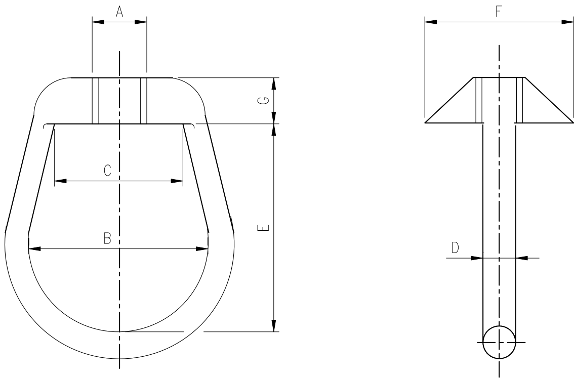
DIMENSIONS (mm)
