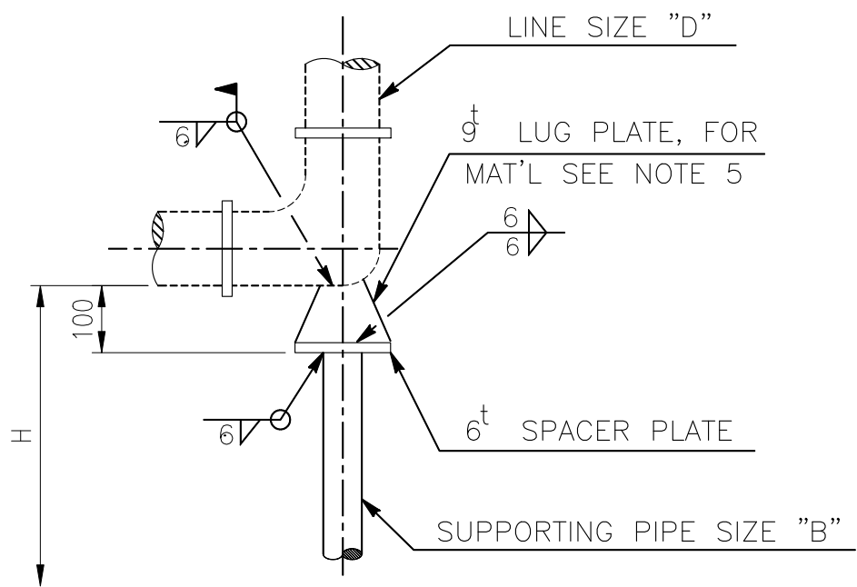
FIG - A
