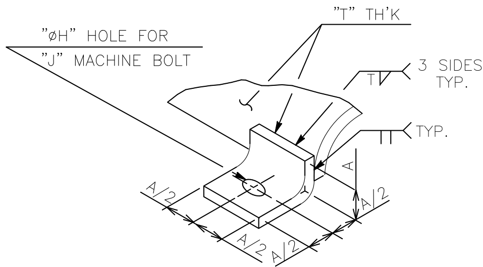
DETAIL "Z"
