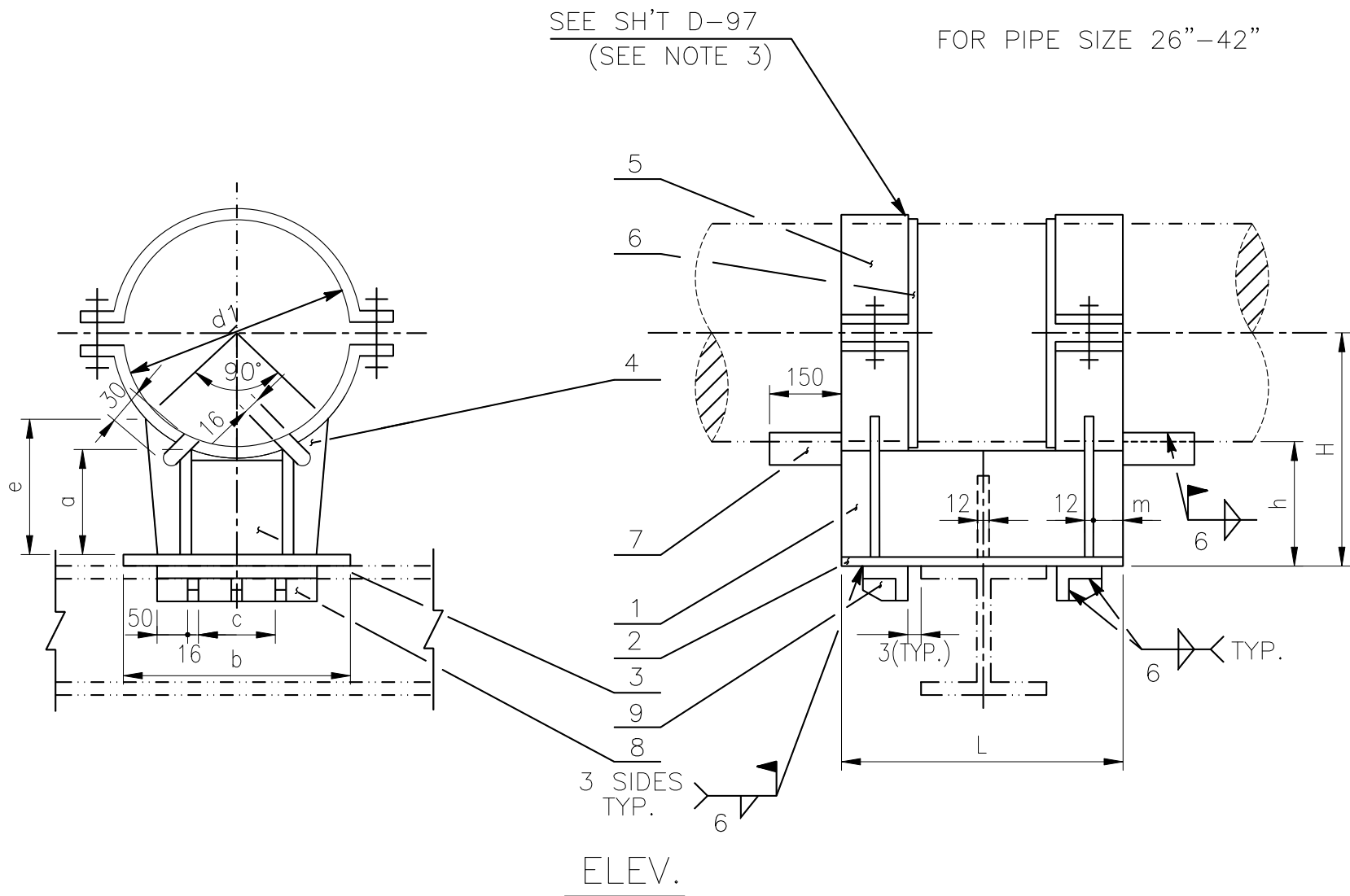
DIMENSIONS (mm)
