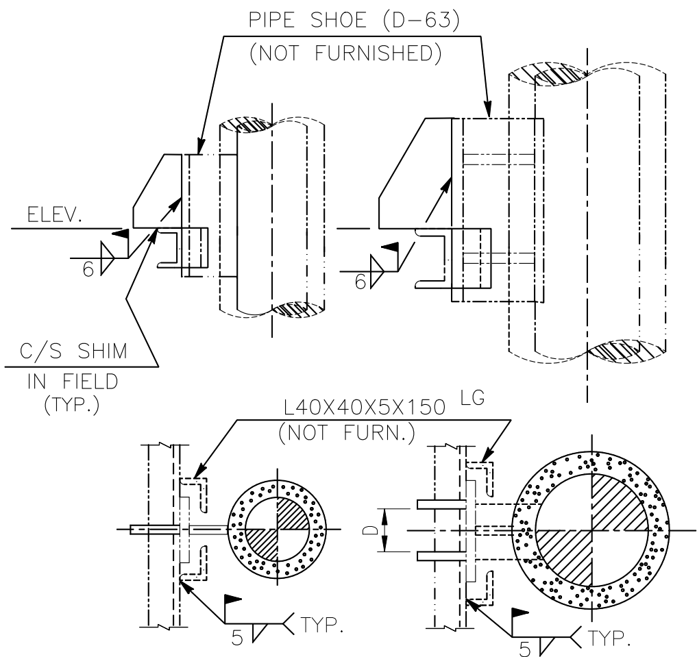
FIG. -A (FOR INS. PIPE)
