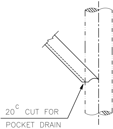
DETAIL "Z" (FOR L-ANGLE ONLY)
